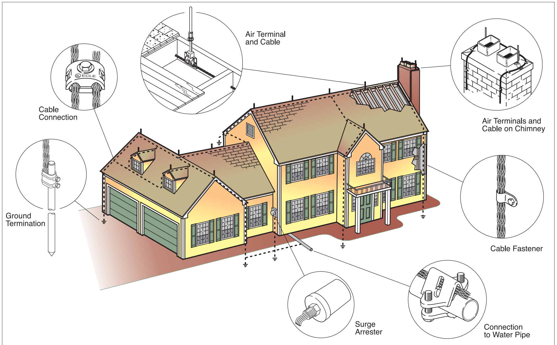
Typical Residential Lightning Protection System
